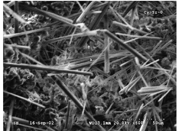
Fig. 5. SEM picture of ASC matrices.
